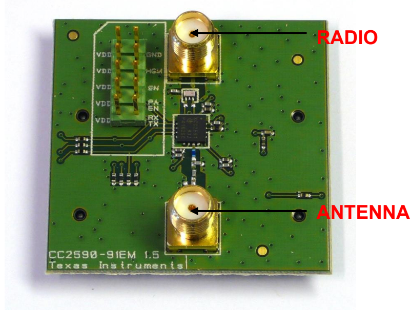
Figure 1 - CC2591EM
