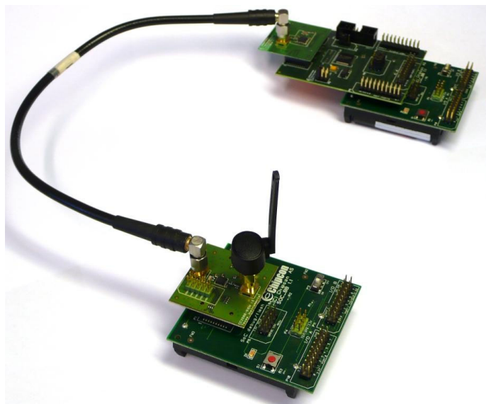
Figure 2 - Possible set up of CC2591 + radio (no control signals)
